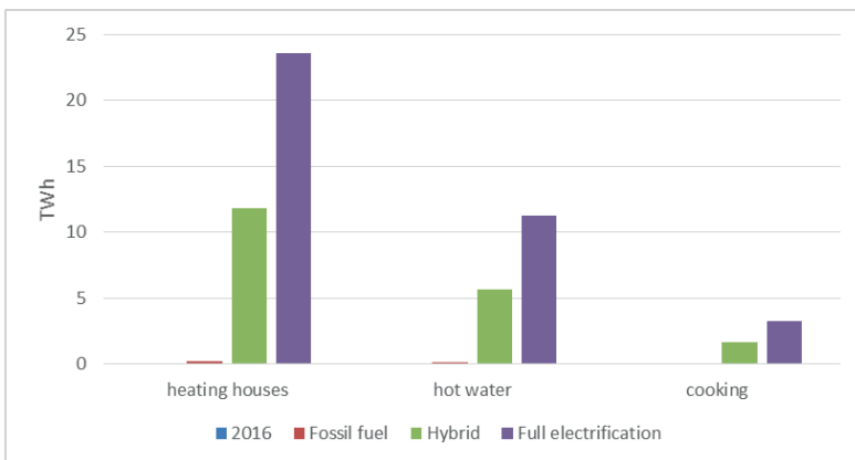
Figure 3.3. Electricity use by residential buildings, per type of use, in 2016 and per scenario in 2050
