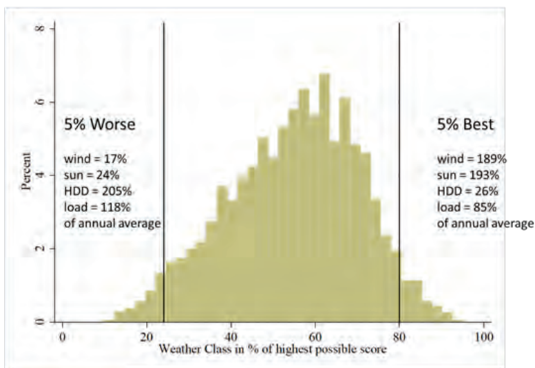
Figure 7.1: Definition of 5% Worse and 5% Best days for electricity system (based on actual data on Dutch market over 2006-2014)
