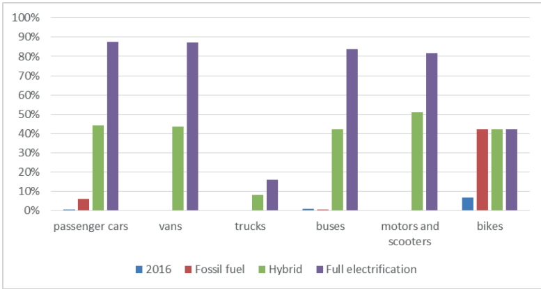
Figure 4.1. Electrification in road transport (in %), by type of vehicle in 2016 and per scenario in 2050
